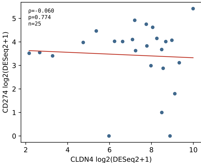
GSE179351 baseline CLDN4 vs CD274
