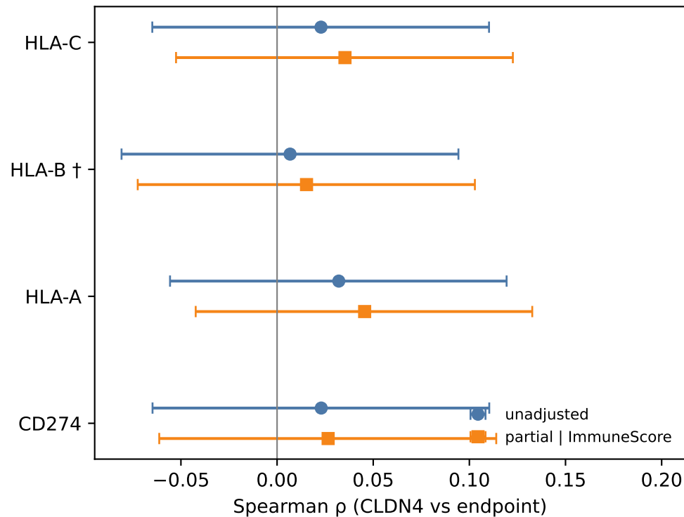
TCGA-LUSC n=501
