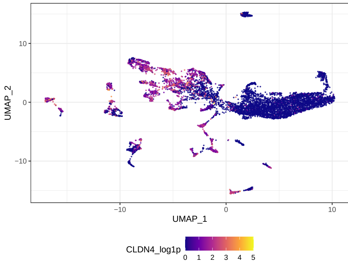
Seurat Harmony UMAP ... CLDN4 (log-norm)
