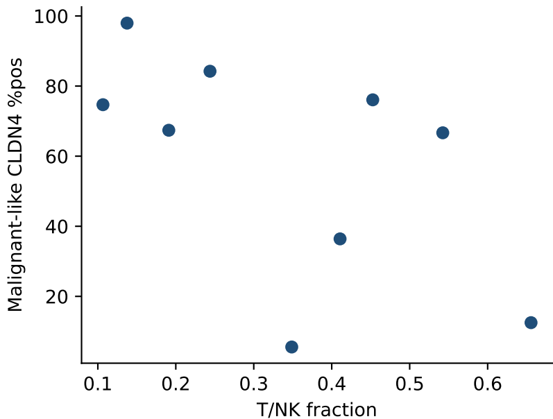
GSE253013 marker_malign / tnk / pct (n=9)
