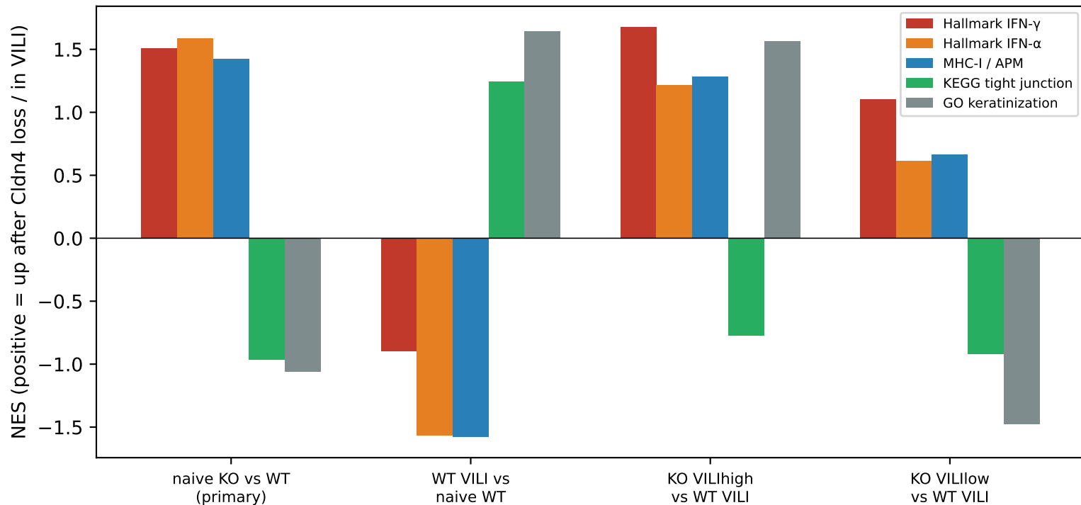
GSE50927 mouse lung — prerank GSEA (n=1 vs 1 per contrast)
