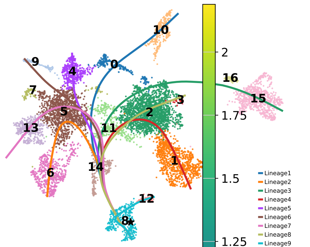
UMAP Leiden + Slingshot curves
