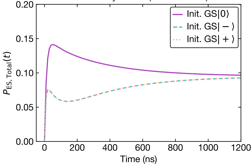
Readout Dynamics ( \Gamma = 12.8 MHz)
