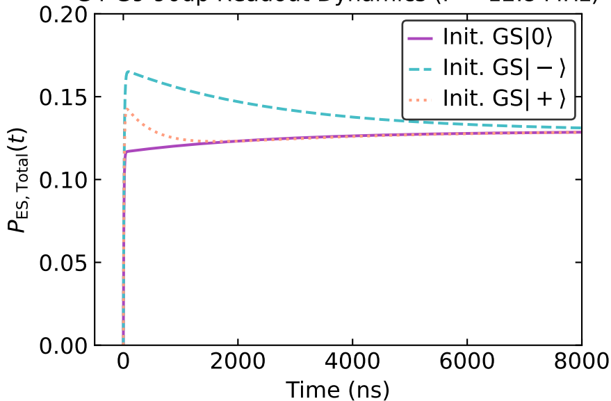
G4-G9 90dp Readout Dynamics ( \Gamma = 12.8 MHz)
