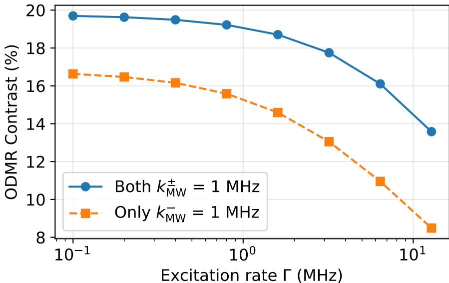
8-Level Model ODMR Contrast
