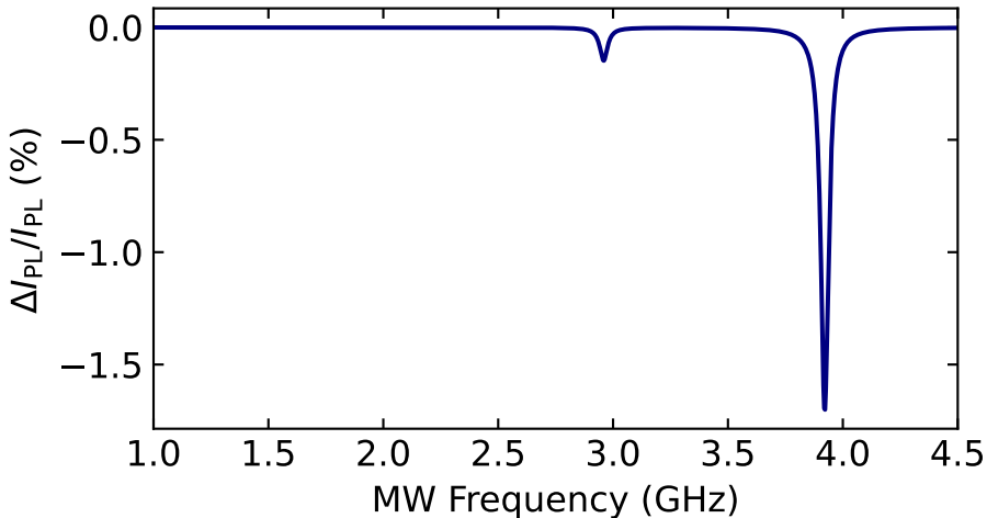
G11-Gm9 30dp ODMR Spectrum (Split Peaks)
