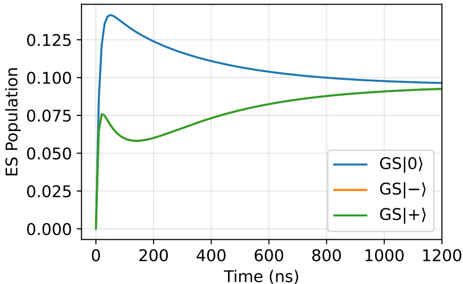
8-Level Readout ( \Gamma = 12.8 MHz)
