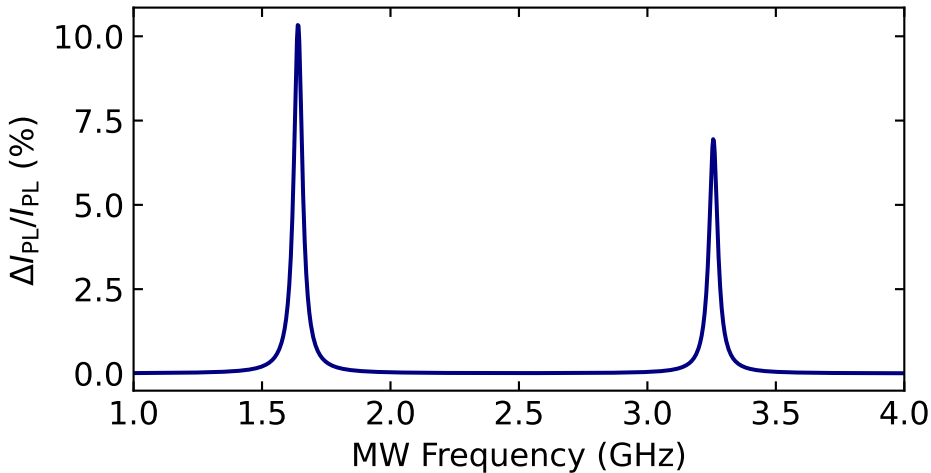
G4-G9 90dp ODMR Spectrum (Split Peaks)
