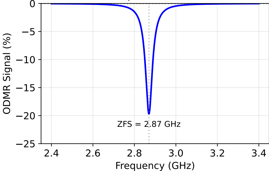
8-Level ODMR Spectrum at ZFS = 2.87 GHz
