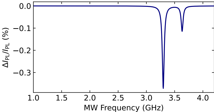
G9-G8 30dp ODMR Spectrum (Split Peaks)
