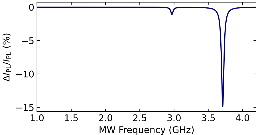
GP7-GP3 30dp ODMR Spectrum (Split Peaks)
