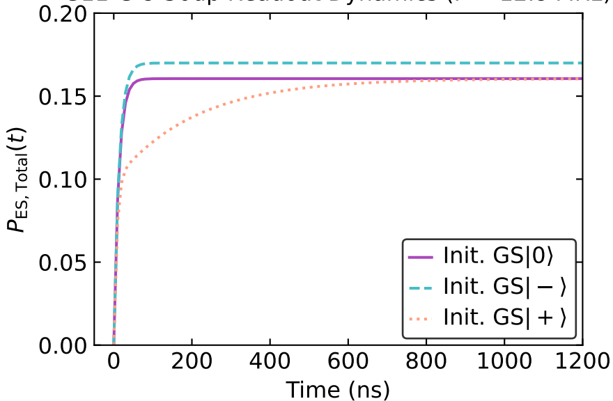
G11-G-9 30dp Readout Dynamics ( \Gamma = 12.8 MHz)
