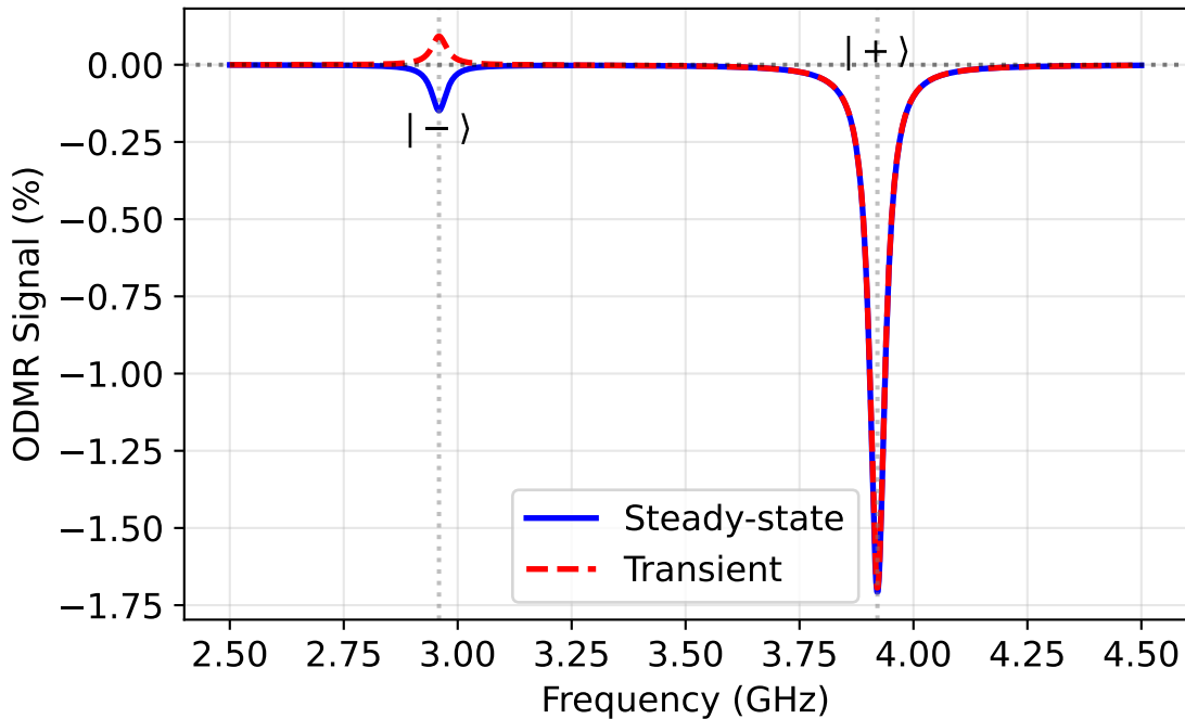
G11-Gm9 30dp ODMR Spectrum ( \Gamma = 0.1 MHz)
