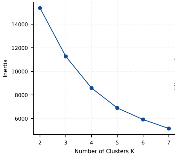
Elbow Method
