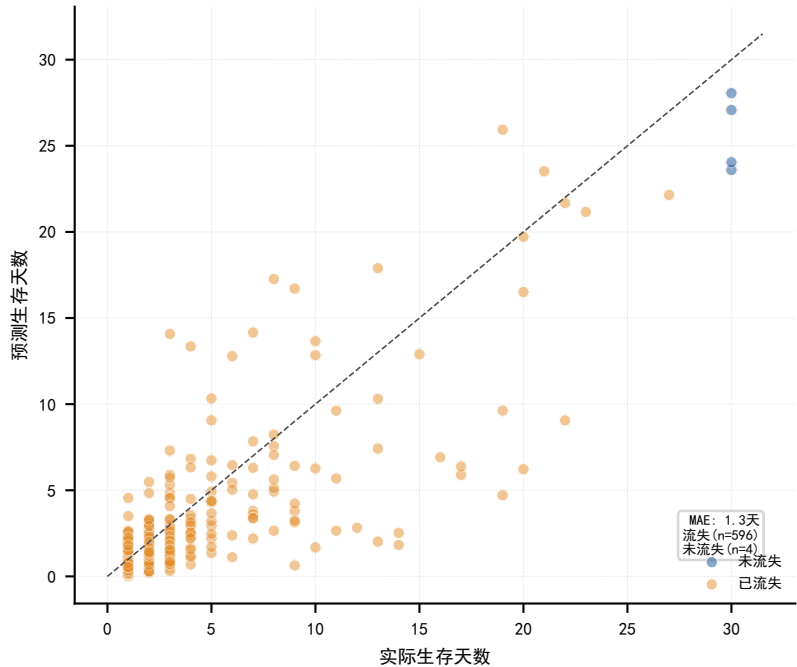
按流失状态分层 (C=0.902)
