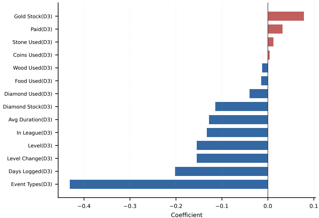
Cox: Day3 Feature Impact on Churn Risk
