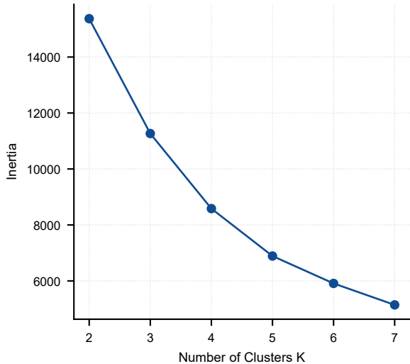
Elbow Method
