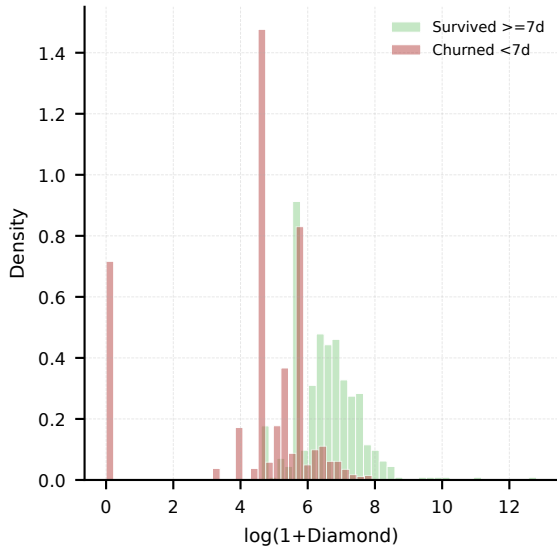
Diamond: Survive vs Churn
