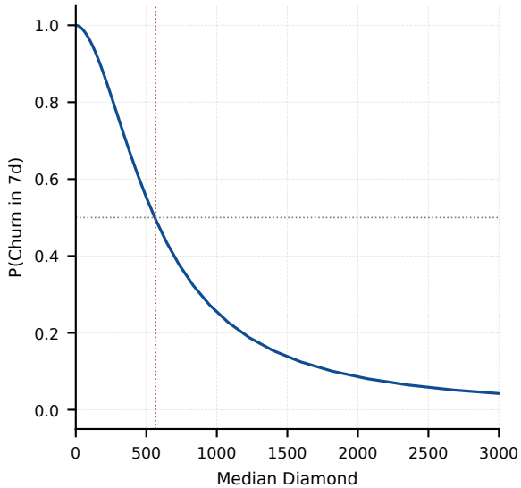
Churn Risk vs Diamond (Thresh \approx 566 )
