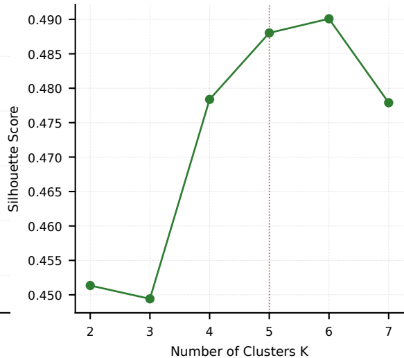
Silhouette Analysis (Best K=5)
