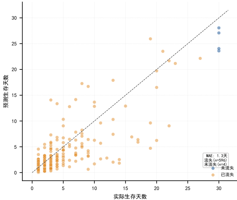
按流失状态分层 (C=0.902)
