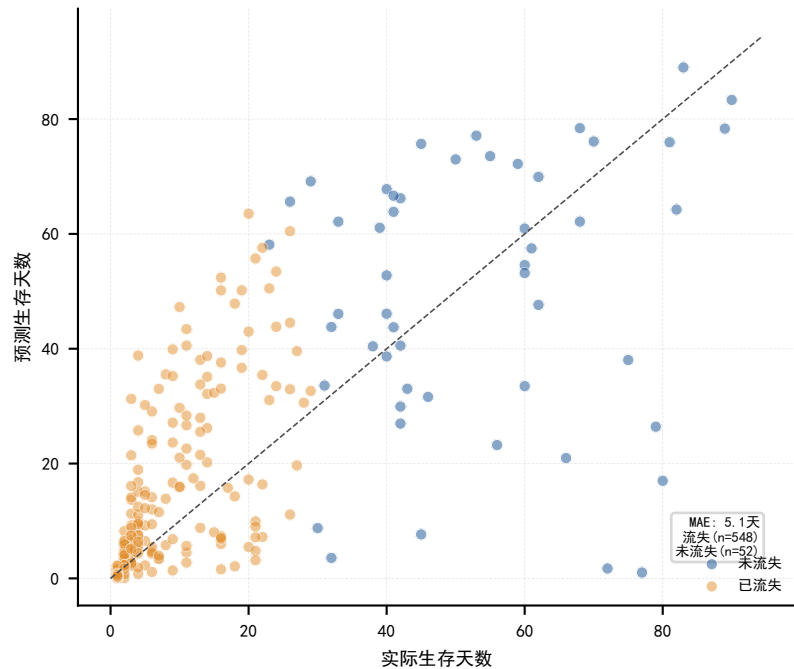
按流失状态分层 (C=0.950)
