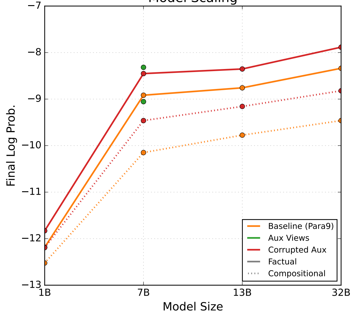
Model Scaling
