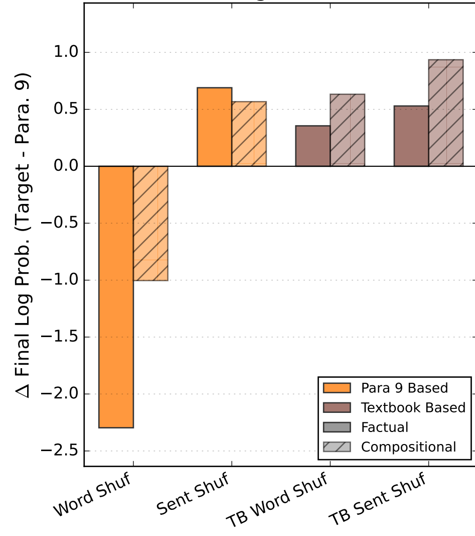
Shuffling Effect (7B)
