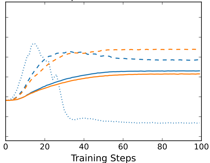
Compositional Probes
