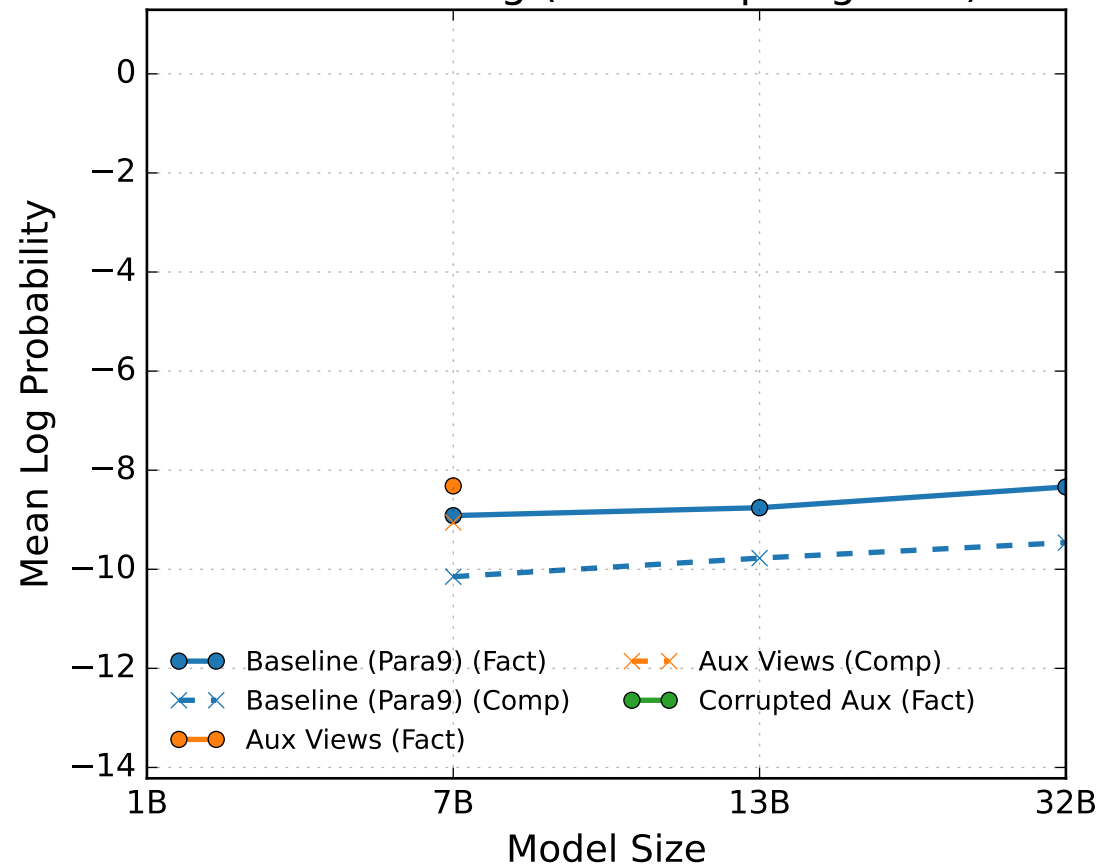
Model Scaling (Final Step Log Prob)
