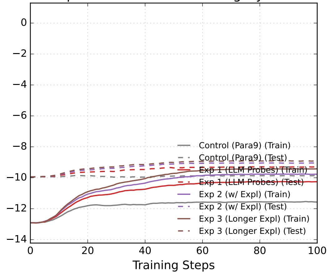
Compositional Probes: Training Dynamics
