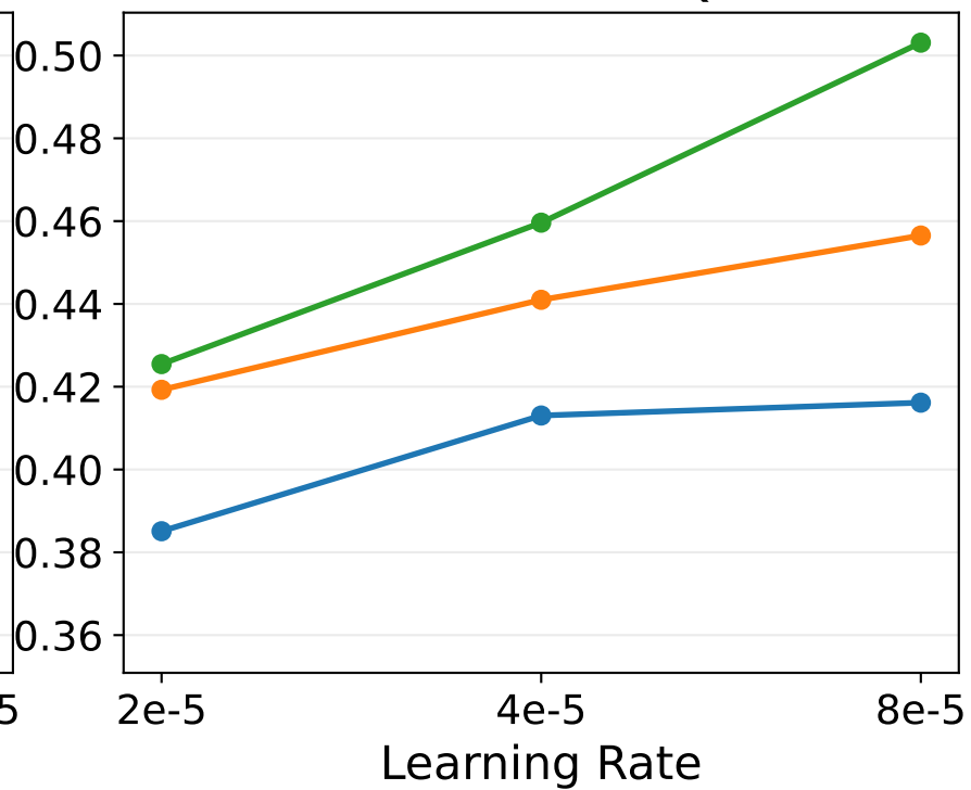
Inference MCQA
