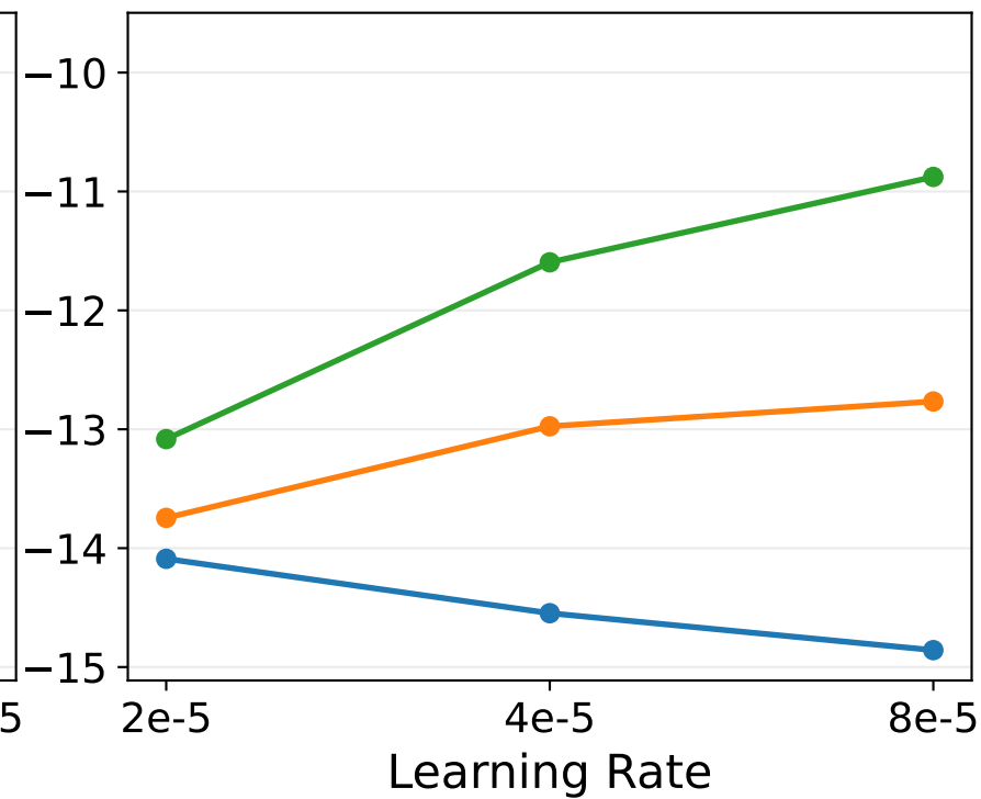
Inference Probes
