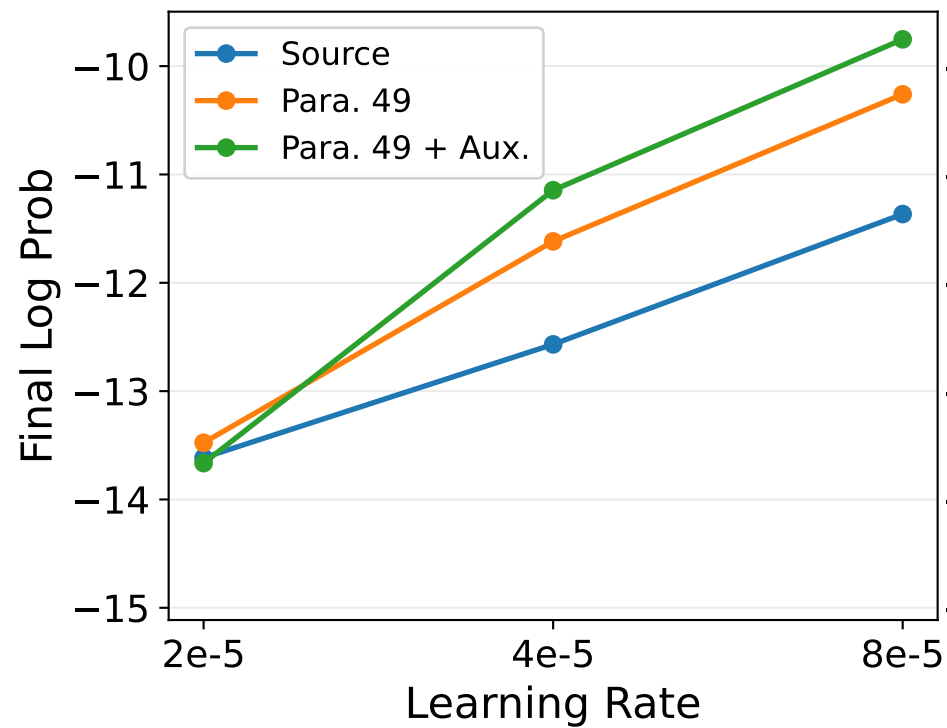
Factual Probes
