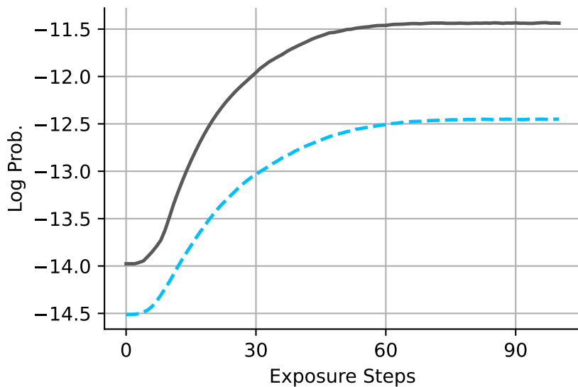
1B: Factual Probes
