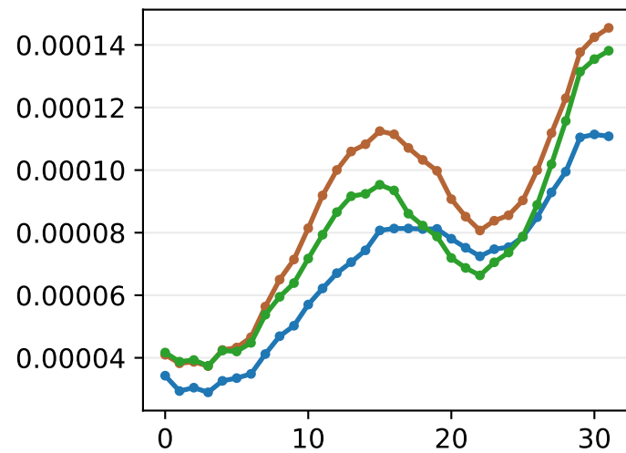
Cosine distance
