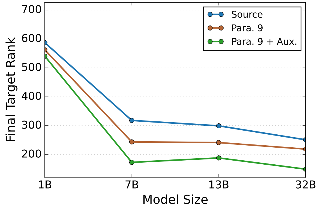
Factual Probes
