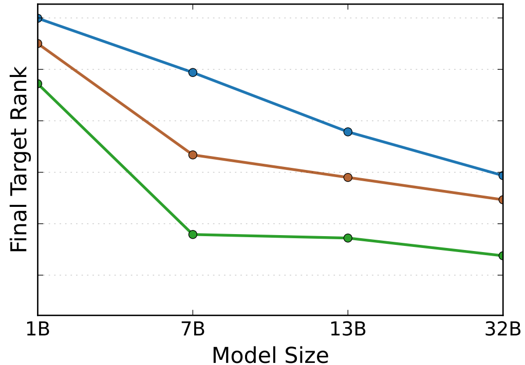
Inference Probes
