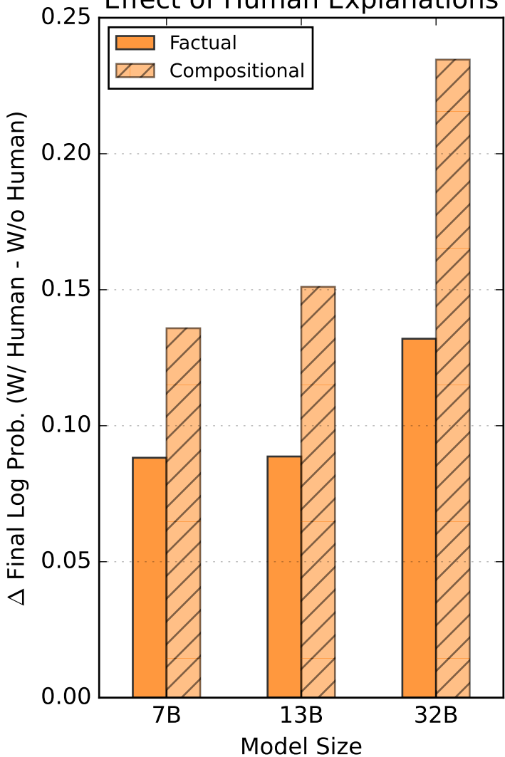
Effect of Human Explanations
