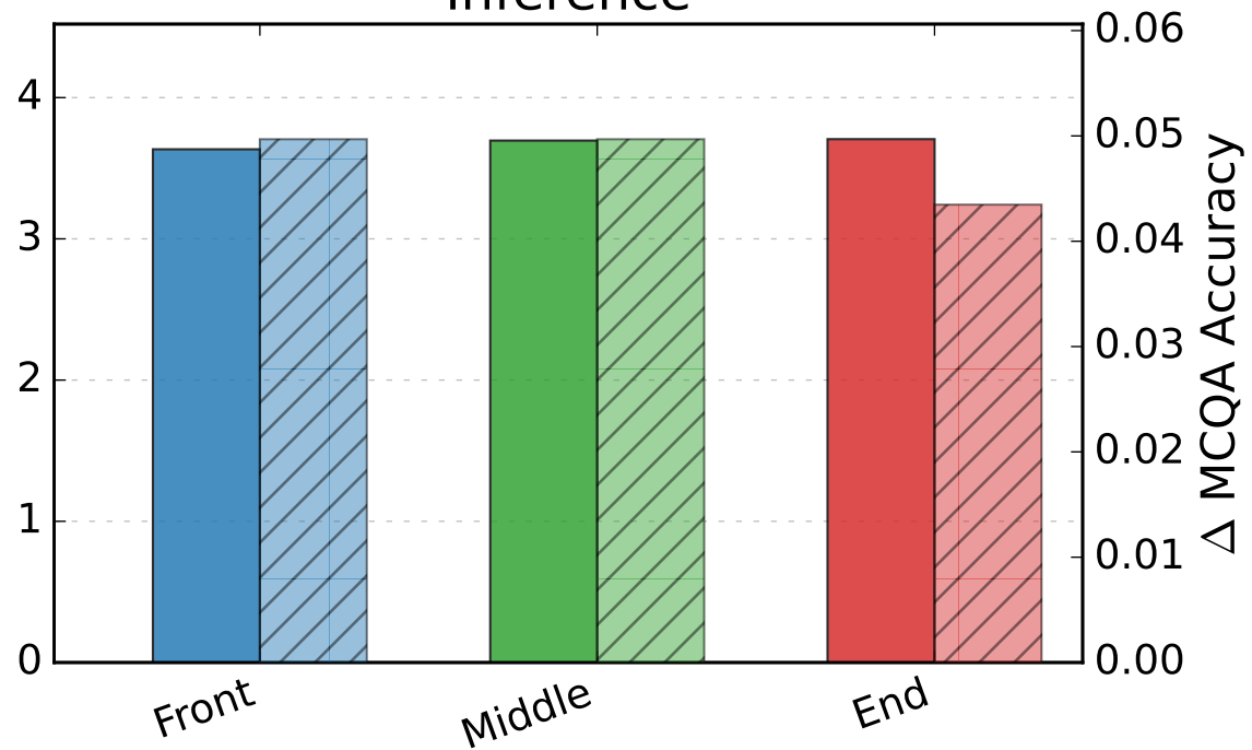
Inference
