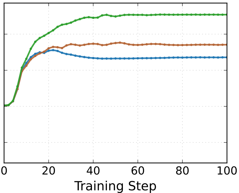
Inference Probes
