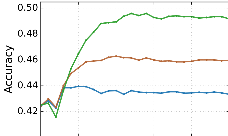
Factual Probes
