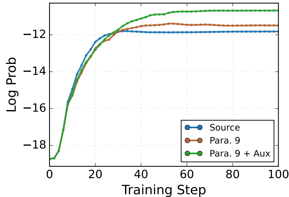
Factual Probes
