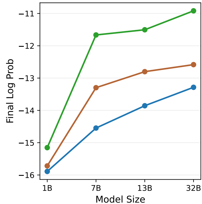
Inference Probes
