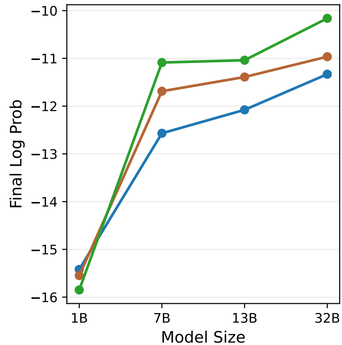
Factual Probes
