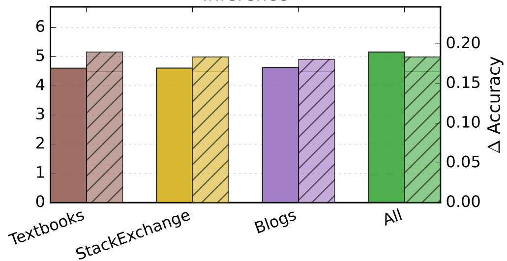
Inference
