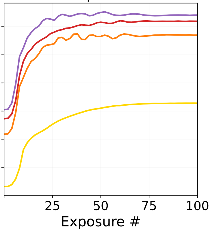
Paraphrased
