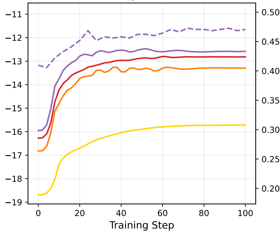
Paraphrased
