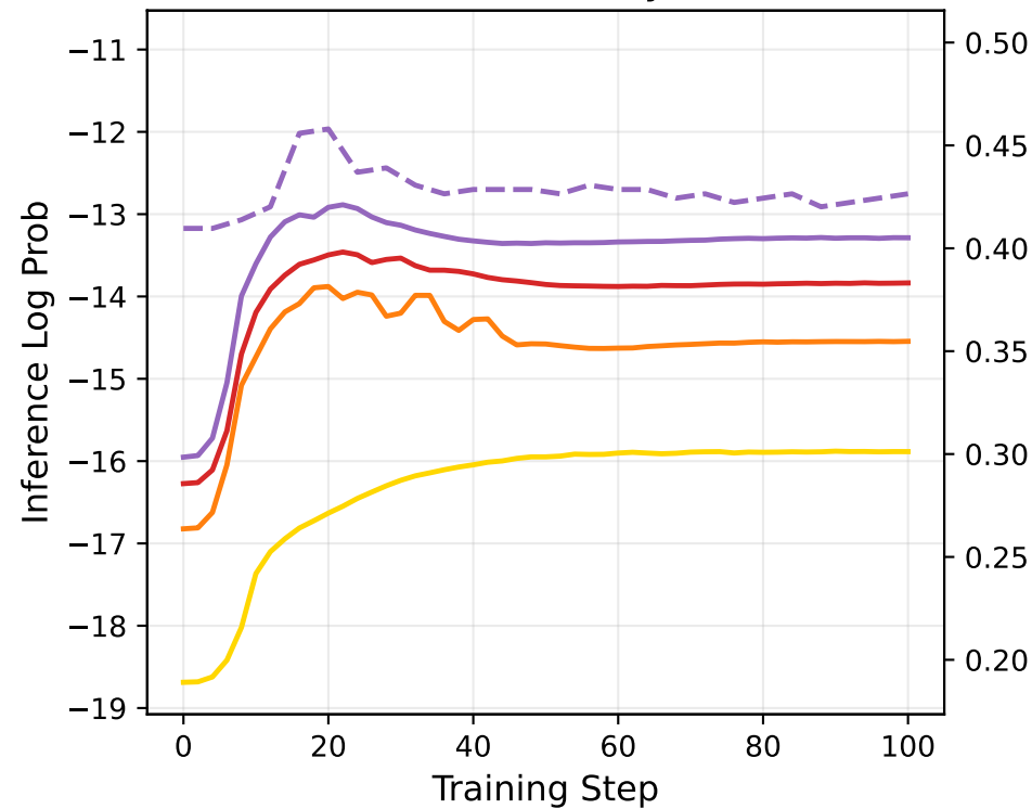
Source Only
