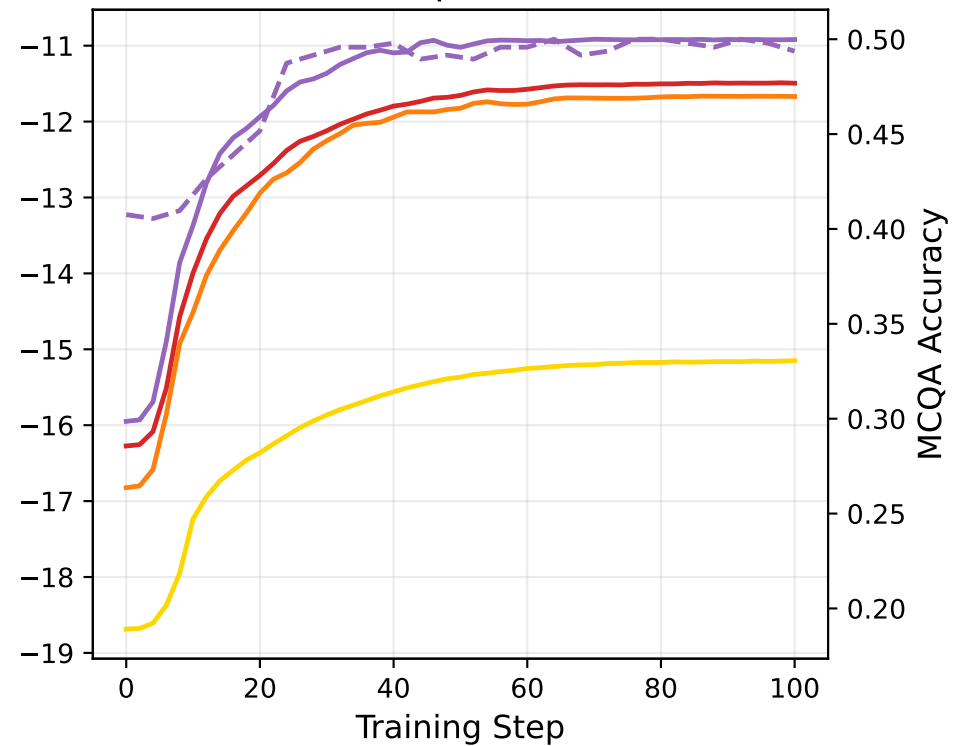
With Explanations
