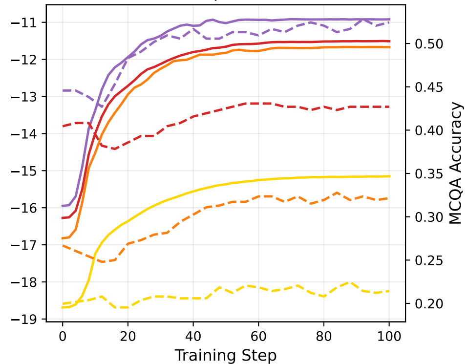
With Explanations
