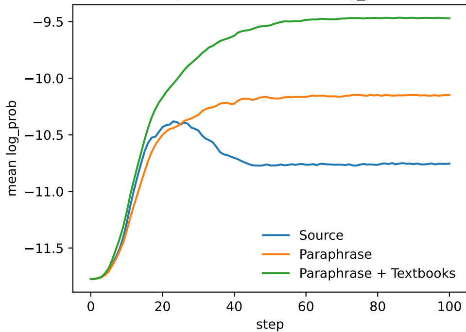
Compositional Probes — log_prob
