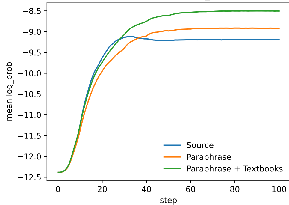
Factual Probes — log_prob
