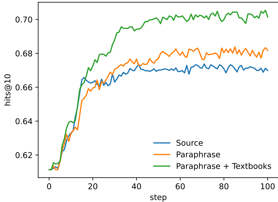
Compositional Probes — hits@10
