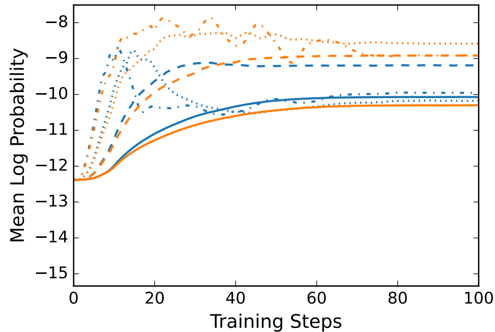
Factual Probes
