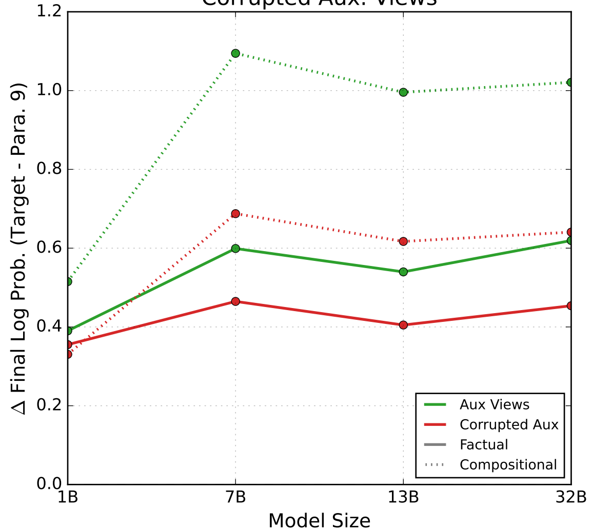
Corrupted Aux. Views
