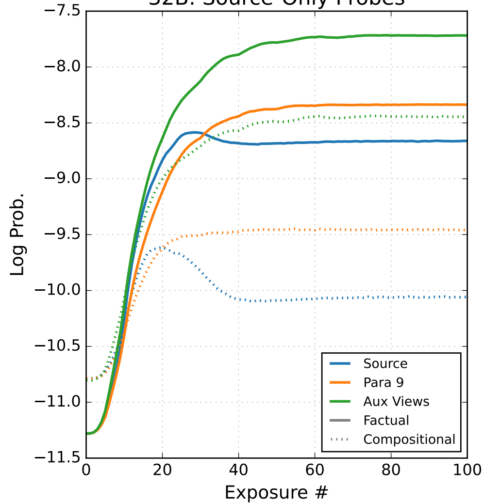
32B: Source-Only Probes
