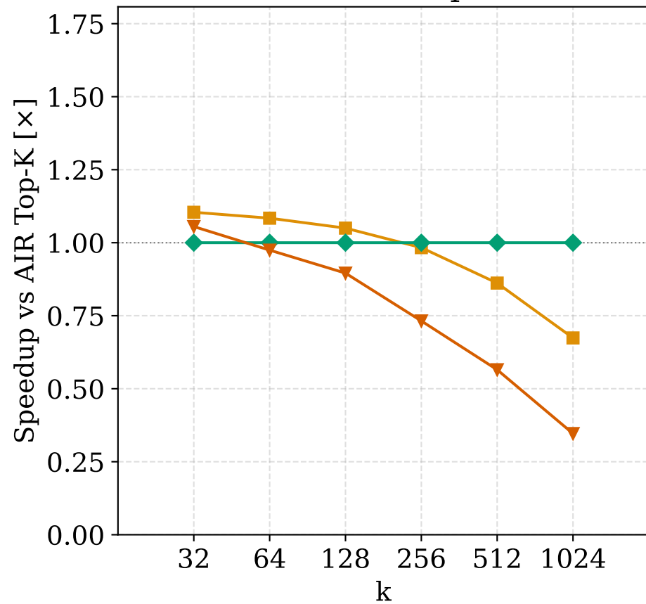
Database top-N
