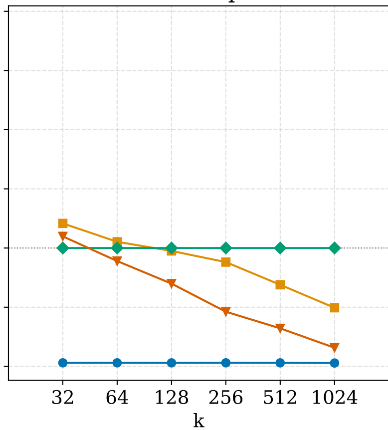
Gradient compression
