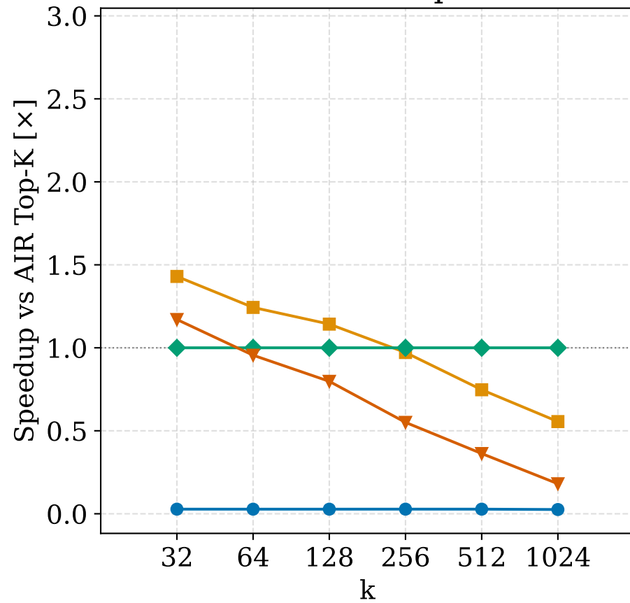
Database top-N
