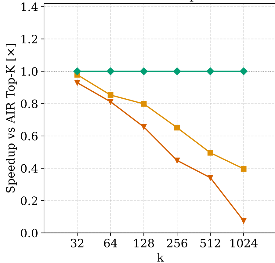
Database top-N
