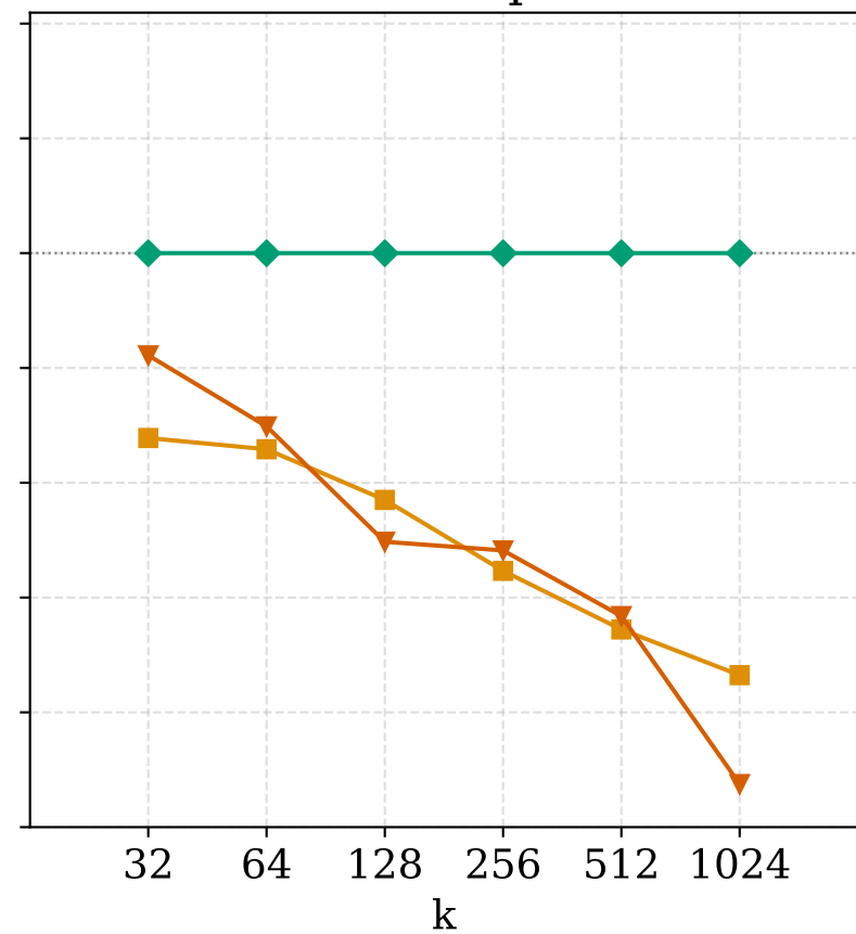
Gradient compression
