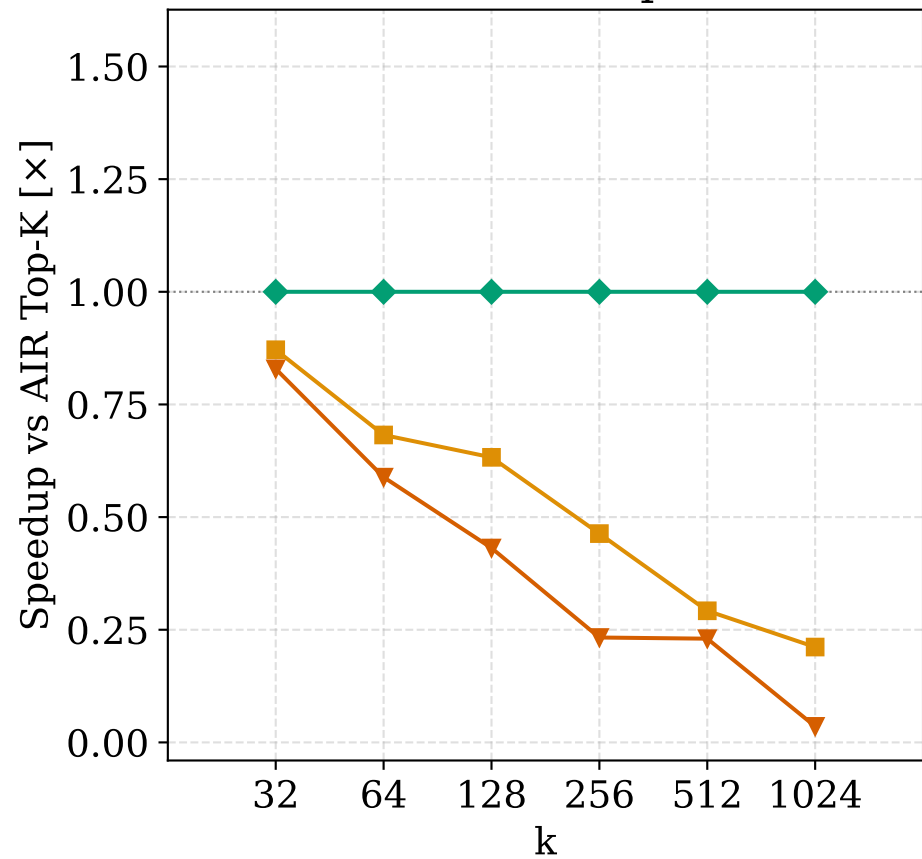
Database top-N
