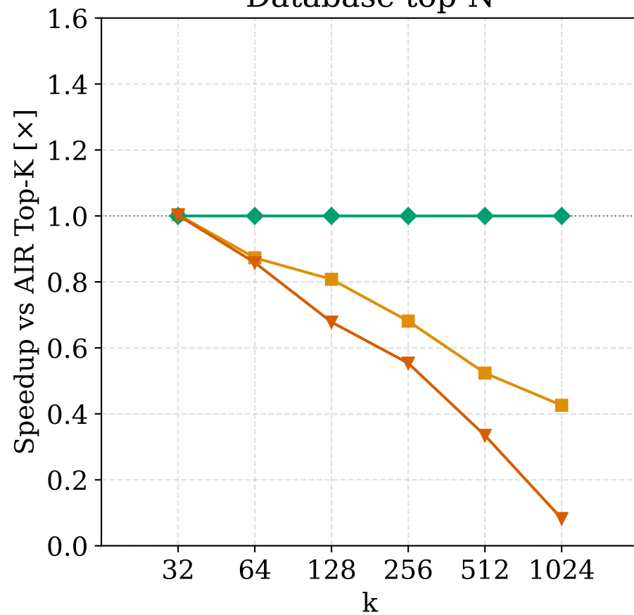
Database top-N
