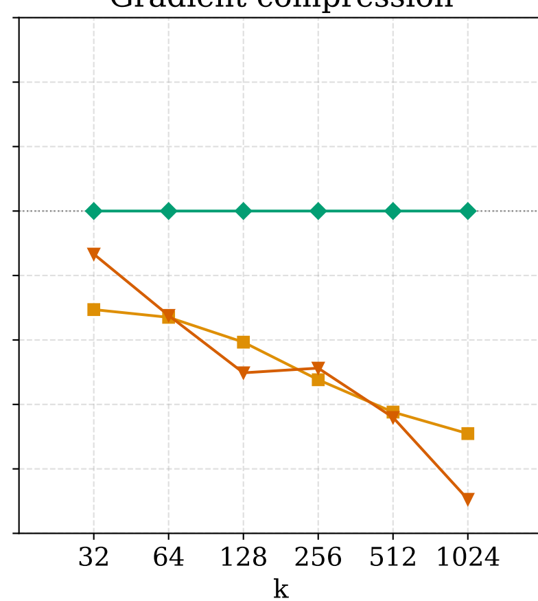
Gradient compression
