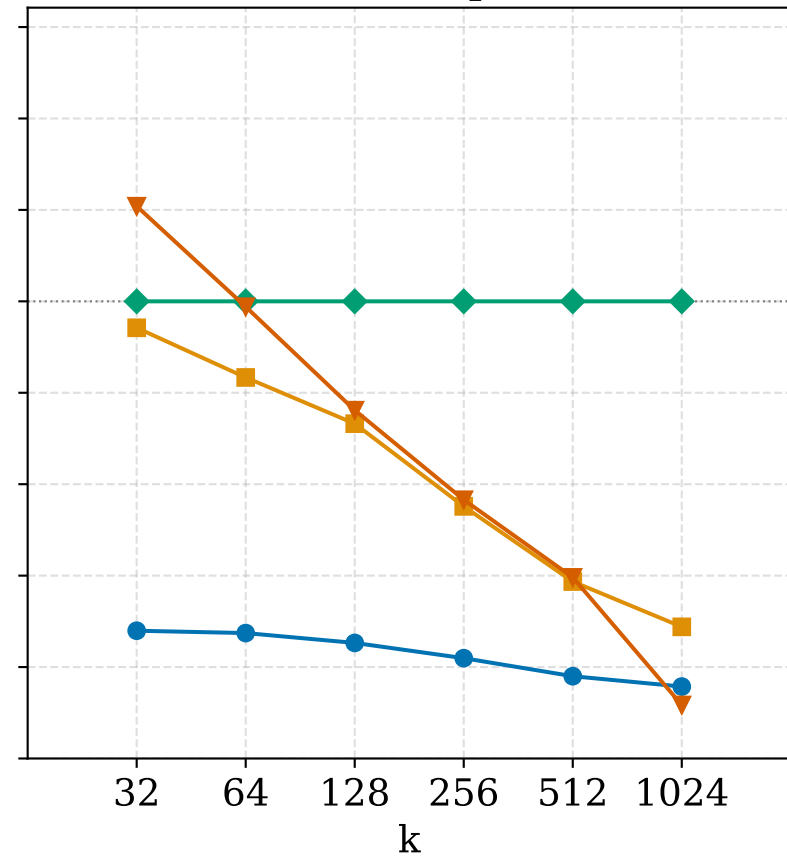
Gradient compression
