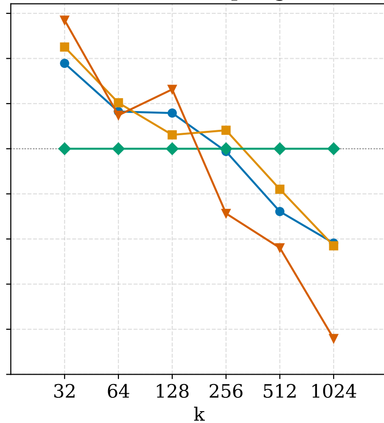
Token sampling
