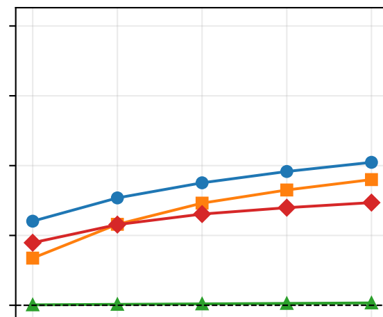
Naive
