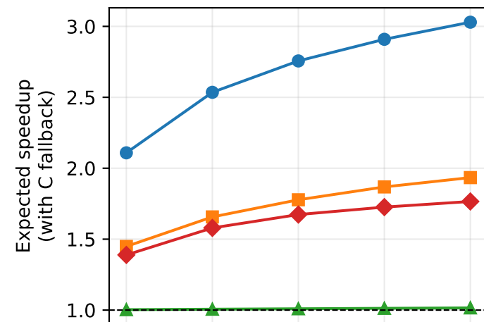
AllHints
