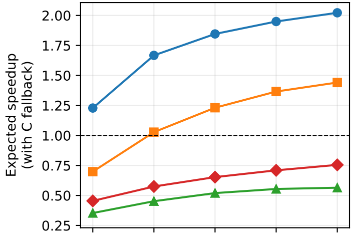
AllHints
