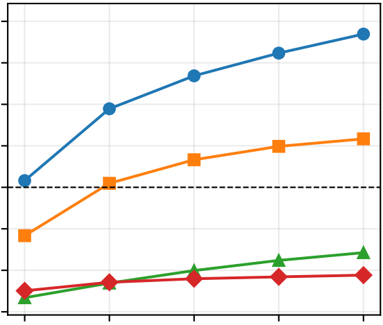
ChooseHints
