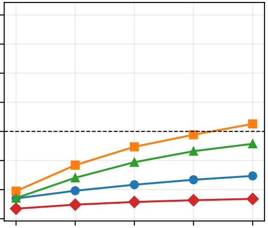
Naive
