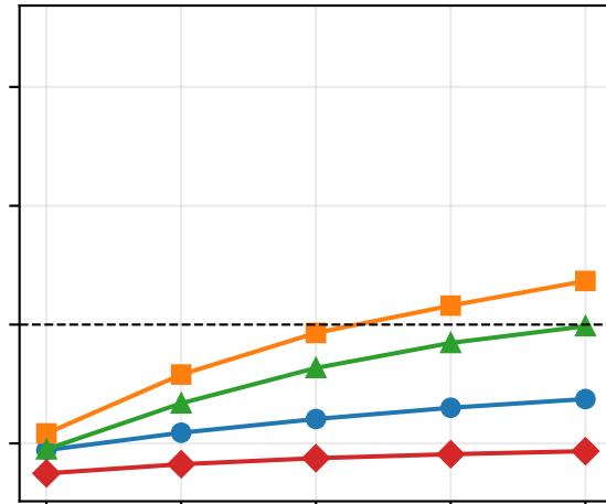
Naive
