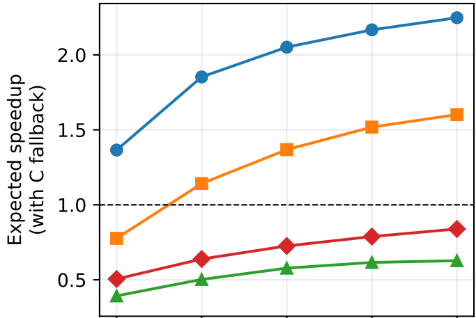
AllHints
