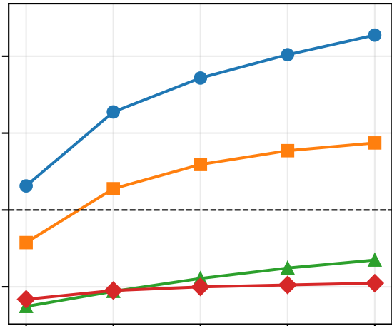
ChooseHints
