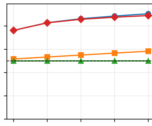
Naive
