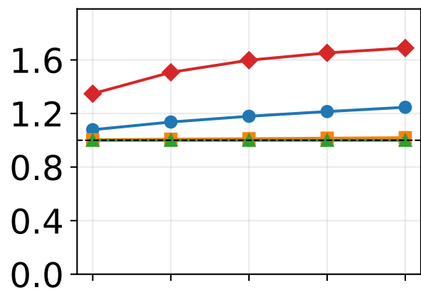
AllHints
