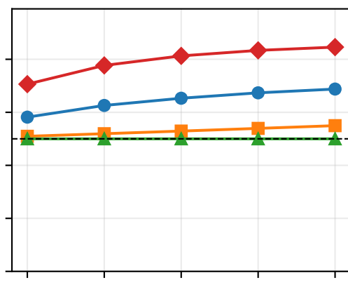
ChooseHints
