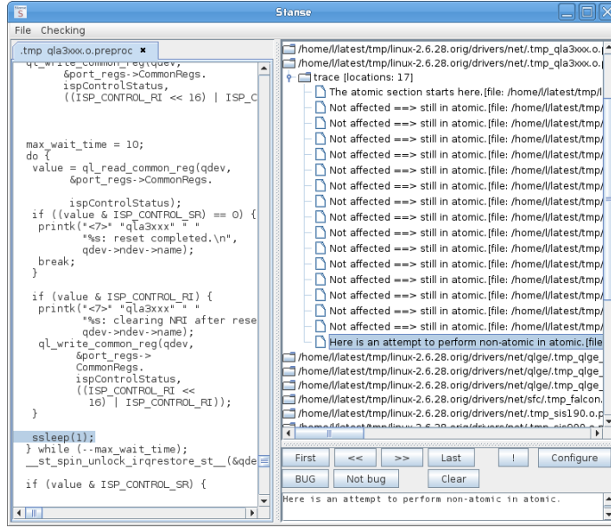
Fig. 1. Error trace browser in the STANSE GUI.
