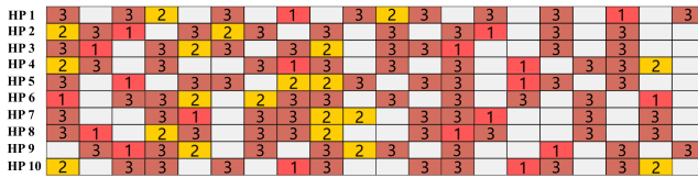
Fig. 2. Scheduling pattern of \Gamma = \{\tau_1(C_1 = 1, T_1 = 10, D_1 = 10), \tau_2(2, 20, 20), \tau_3(2, 5, 5)\} scheduled by dynamic-priority scheduling and with scheduling randomization on a uniprocessor platform.
