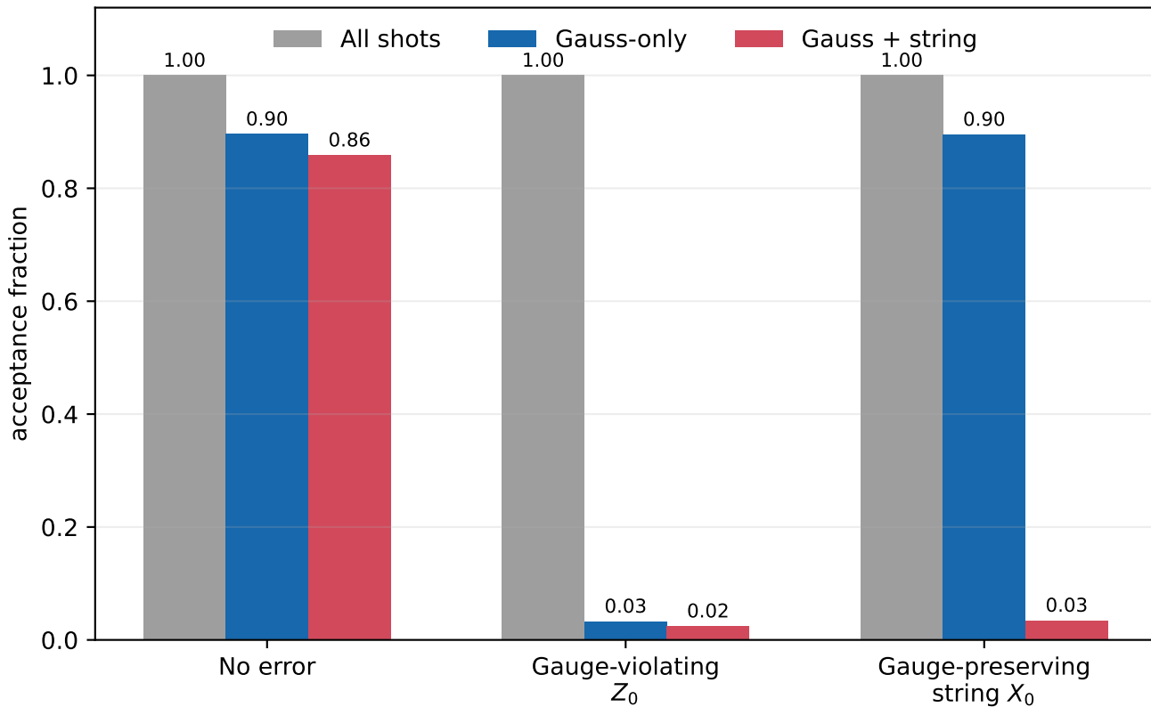
String-aware selection rejects the Gauss-preserving error
