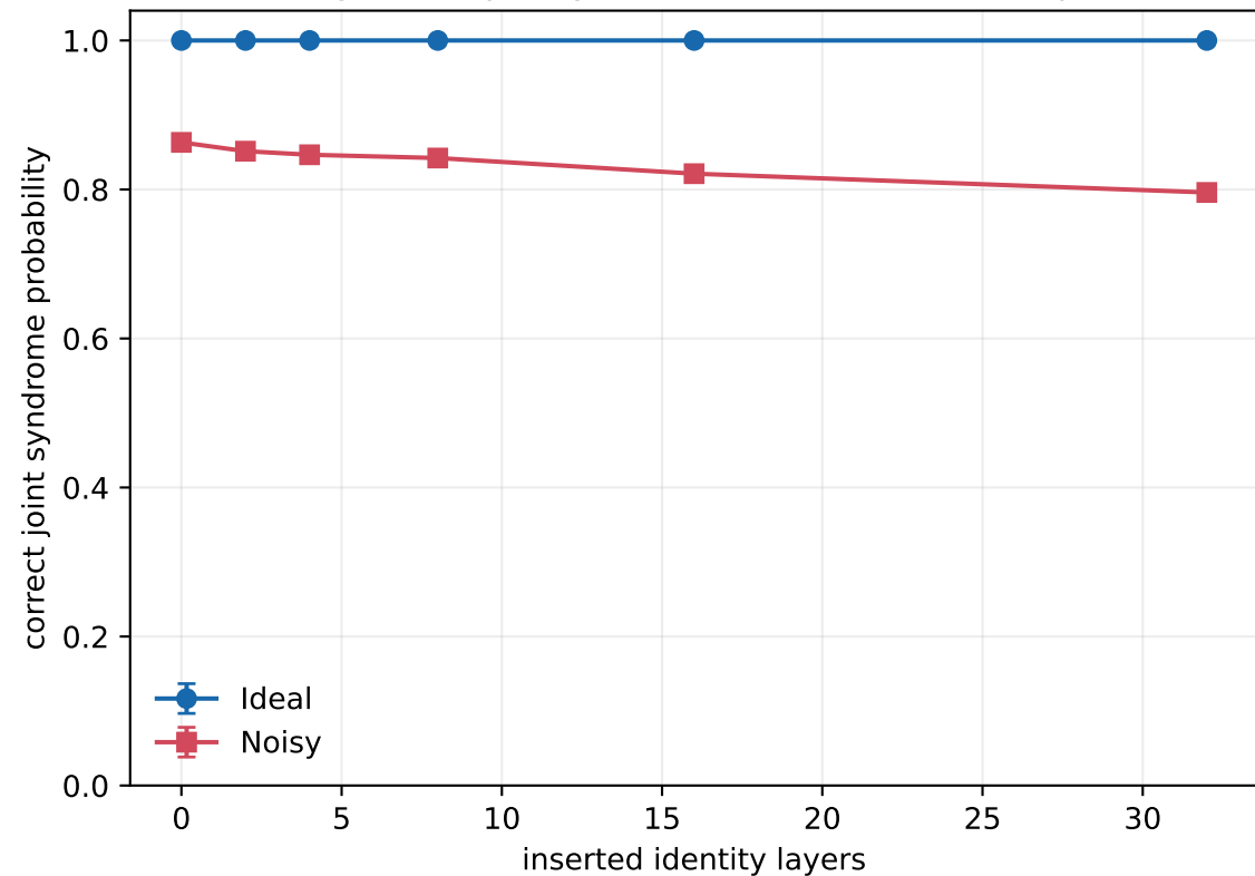
Diagnostic quality versus inserted circuit depth
