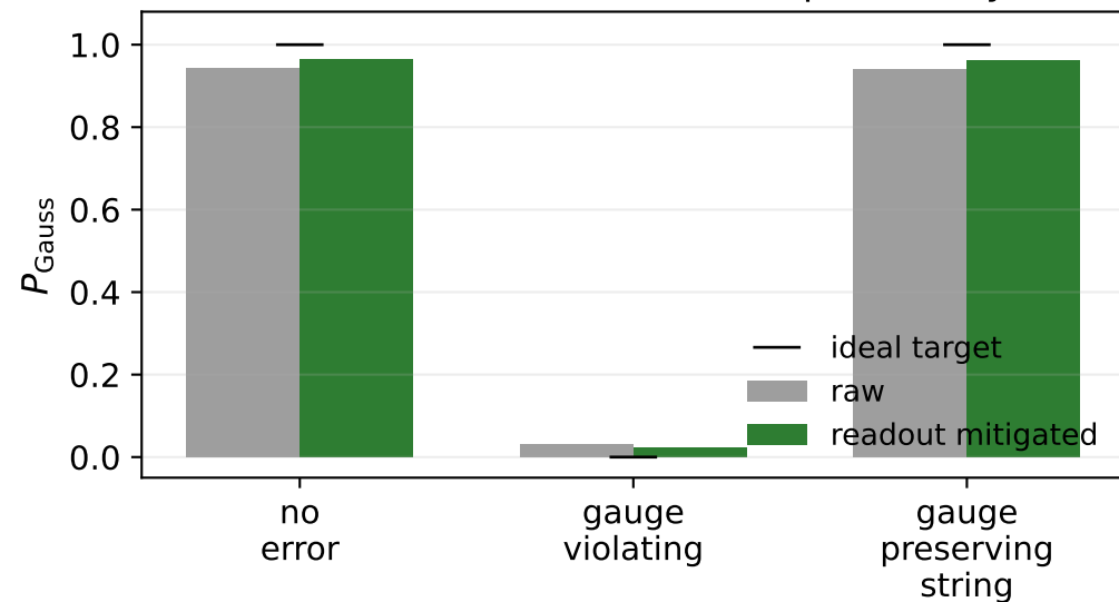
Periodic Emerald: readout correction is modest
