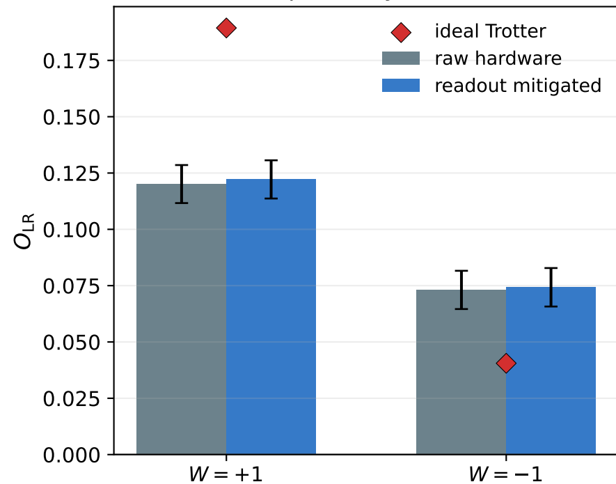
Matter response by Wilson sector
