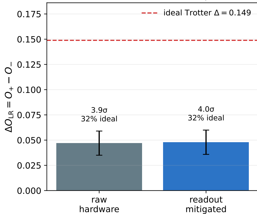
Resolved hardware sector separation
